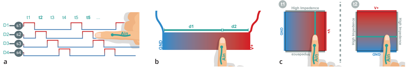
Figure 4: Electrical principles used for touch sensing (a), linear position sensing (b), and gesture sensing (c).
